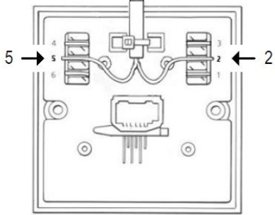
On-site BT Socket
