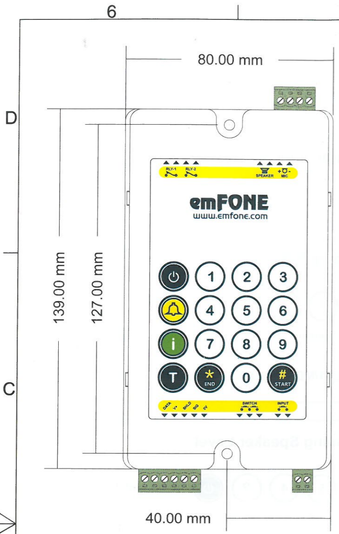
FRONT VIEW
